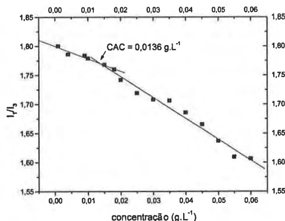
Figure 1. I_1/I_3 ratio of the vibronic band intensities of pyrene ( 1 \times 10^{-6} \text{ mol.L}^{-1} ) as a function of substituted chitosan concentration:
